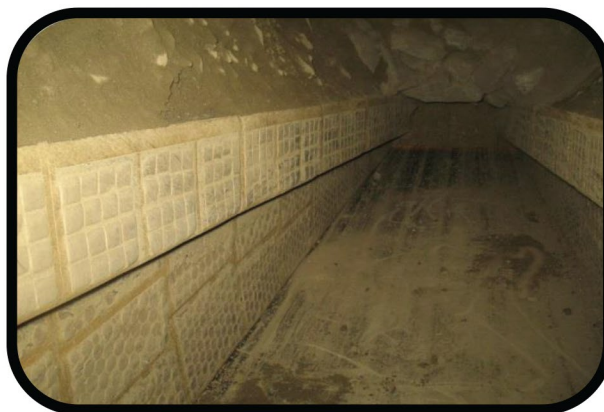
Existing loading shoe in a 60" Feeder taken at 50 weeks
