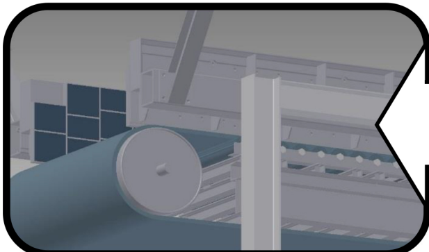
Total assembled weight of the structural elements is approximately 13,000 lbs. per feeder system
